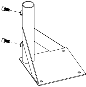
C101-207 4 pole freestander bottom, white powder coated, with screws & clamps
